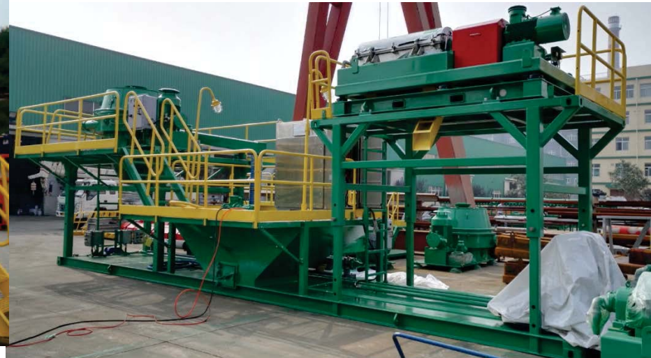
ATEX Zone 1/Zone 2 Certified DWM System For Europe
